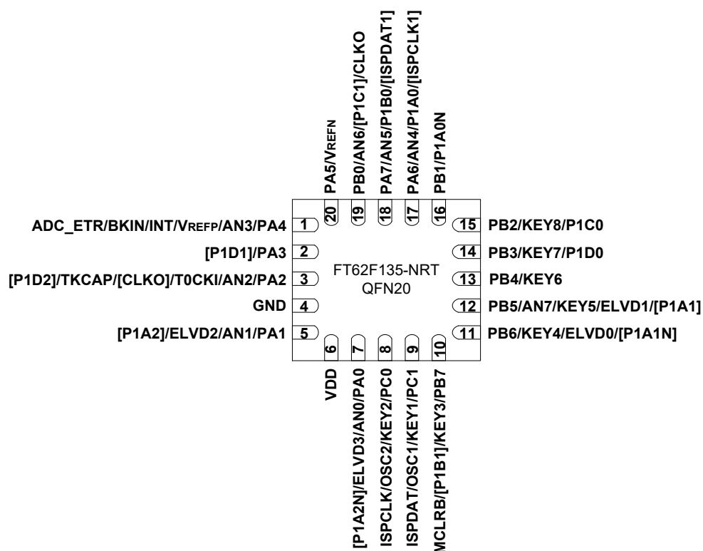
图 1-7 QFN20 2
