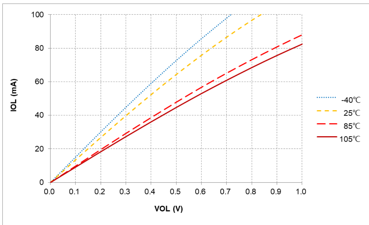
图 19-11 I_{OL} vs. V_{OL} @ L2 = 55\text{mA} , V_{DD} = 5\text{V}
